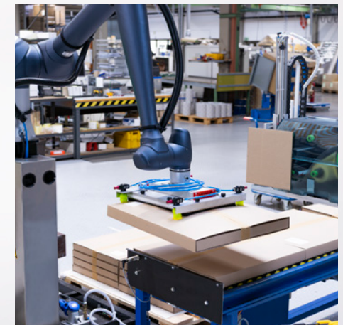
Packaging robot
