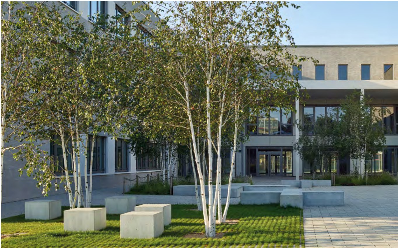
GDM.GREEN stone proActive 40/40/10 cm, nativo, Grau, proDrain und GDM.SCENIC stone 45/15/10 cm, nativo, Granit-Gelb
